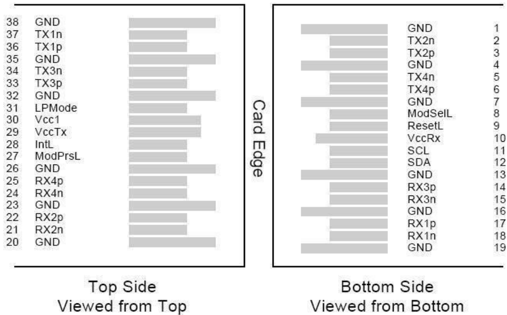
Figure 2: Pin Definitions
