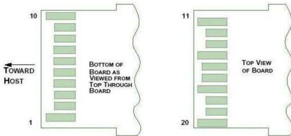
Figure 2: Pin Definitions
